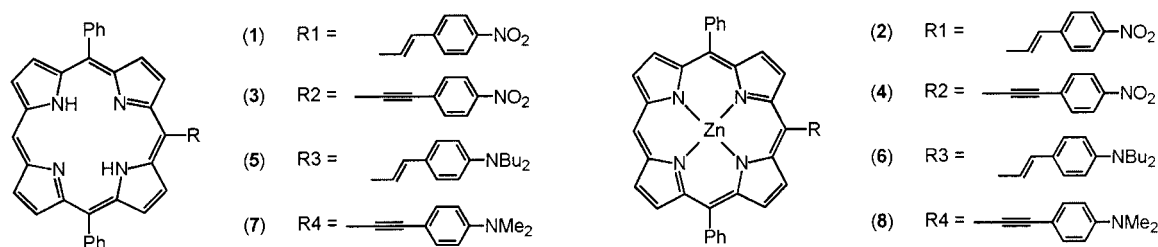
Figure 1. Asymmetrical 10,20-diphenylporphyrins and their Zn II complexes substituted at the meso position with electron-withdrawing or electron-donor groups.
