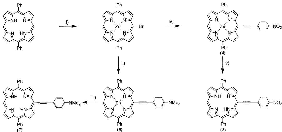
Scheme 2. i) NBS, \text{CHCl}_3 , room temp., 30 min.; \text{Zn}(\text{OAc})_2 \cdot 2\text{H}_2\text{O} , \text{CHCl}_3/\text{MeOH} , reflux, 1 h; ii) catalyst (see Exp. Sect.), [4-(dimethylamino)phenyl]acetylene, pyridine, toluene, 80^\circ\text{C} , 1.5 h; iii) TFA, \text{CH}_2\text{Cl}_2 , 18 h; iv) catalyst (see Exp. Sect.), (4-nitrophenyl)acetylene, pyridine, toluene, 80^\circ\text{C} , 1 h; v) TFA, \text{CH}_2\text{Cl}_2 , 18 h.
