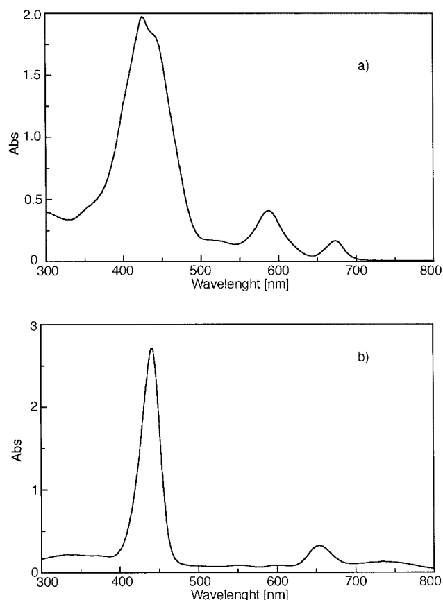
Figure 4. (a) Electronic absorption spectrum of 7 in \text{CHCl}_3 , (b) Electronic absorption spectrum of 7 in \text{CHCl}_3 with the addition of trifluoroacetic acid.
