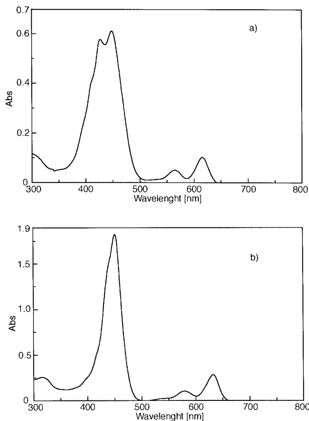
Figure 3. (a) Electronic absorption spectrum of 8 in \text{CHCl}_3 , (b) Electronic absorption spectrum of 8 in \text{CHCl}_3 with the addition of pyridine.
