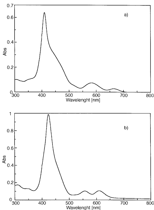
Figure 2. (a) Electronic absorption spectrum of 5 in \text{CHCl}_3 , (b) Electronic absorption spectrum of 6 in \text{CHCl}_3 .
