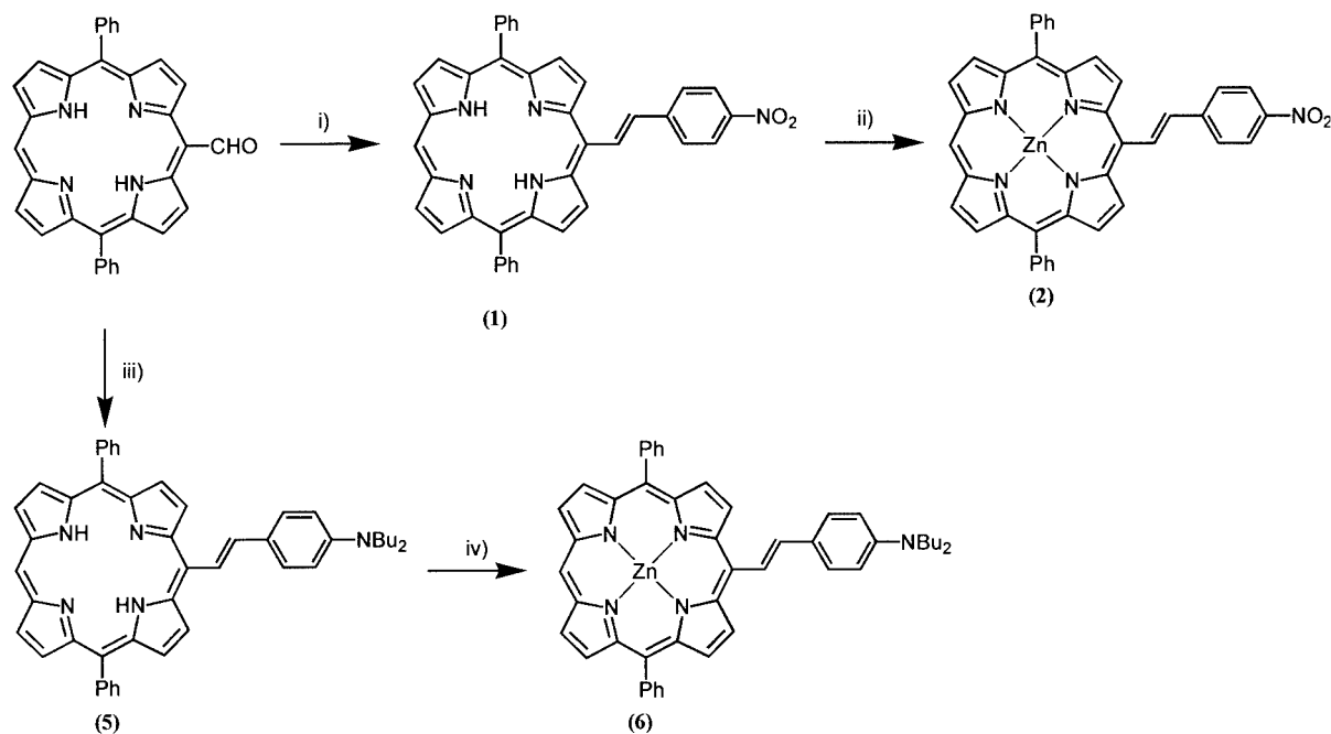
Scheme 1. i) 4-Nitrobenzyltriphenylphosphonium bromide, NaOH, CH 2 Cl 2 , reflux, 4 h; ii) Zn(OAc) 2 ·2H 2 O, CHCl 3 /MeOH, reflux, 1 h; iii) 4-(Dibutylamino)benzyltriphenylphosphonium chloride, NaOH, CH 2 Cl 2 , room temp., 4 h; iv) Zn(OAc) 2 ·2H 2 O, CHCl 3 /MeOH, reflux, 1 h.
